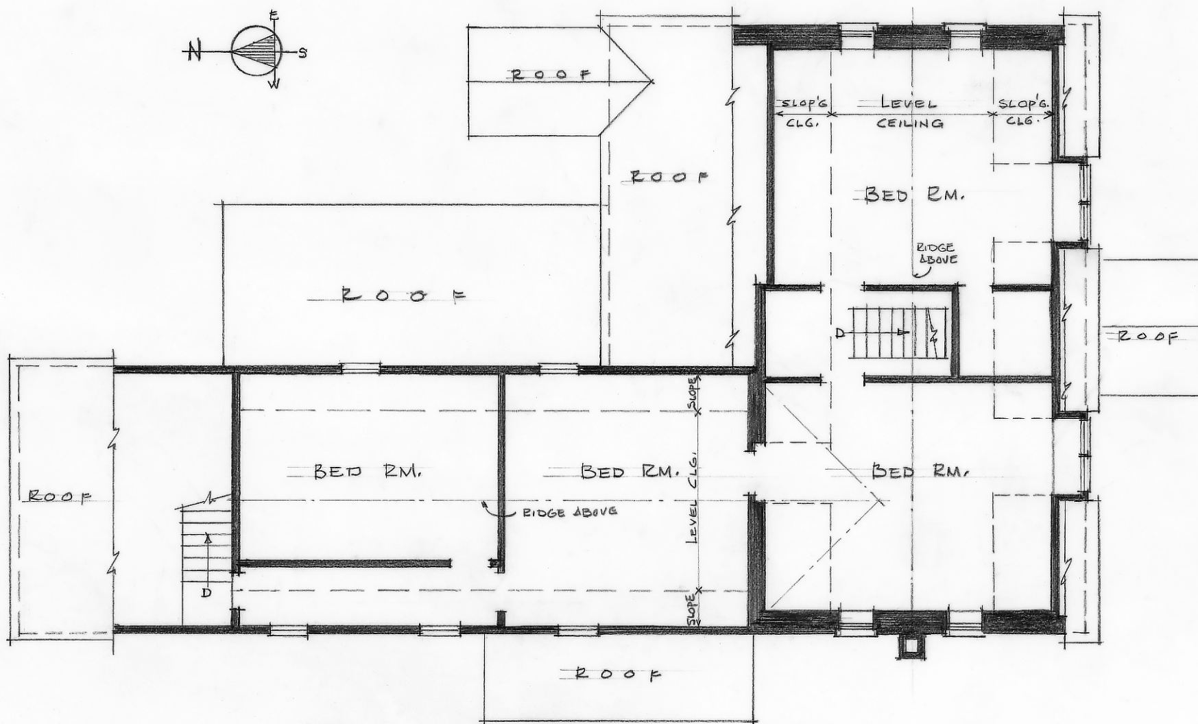
SECOND FLOOR PLAN 1/8" = 1'
